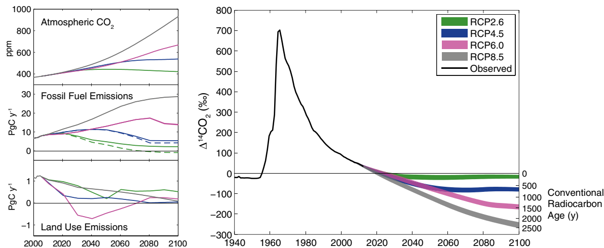
Fig. 1. Model predictions of atmospheric radiocarbon for the RCPs. (Left) Atmospheric \text{CO}_2 concentration (Top), \text{CO}_2 emissions from fossil fuel combustion (Middle), and \text{CO}_2 emissions from land use change (Bottom) in the RCP scenarios (11, 34). (Middle) Fossil fuel \text{CO}_2 emitted to the atmosphere is shown with solid lines; dashed lines show net fossil fuel \text{CO}_2 emitted, including “negative emissions” from biomass energy with carbon capture and storage. (Right) Observed (7, 10, 18, 35, 36) (1940–2012) and projected (2005–2100) radiocarbon content of atmospheric \text{CO}_2 ( \Delta^{14}\text{CO}_2 ) (Table S2). The right axis shows the conventional radiocarbon age of a carbon-containing specimen with the same radiocarbon content, calculated by 8033 \times \ln(\Delta^{14}\text{C}/1,000 + 1) . Filled areas indicate the range simulated for different sets of model parameters, each consistent with 20th-century atmospheric and oceanic \Delta^{14}\text{C} and \text{CO}_2 observations, within their uncertainties (10) (SI Text).
